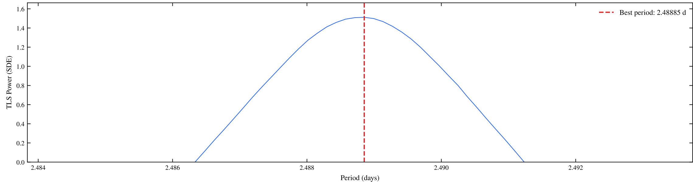
TIC 409934330 | Sectors: 93, 94 | TLS Fine Periodogram (SDE = 1.51)
