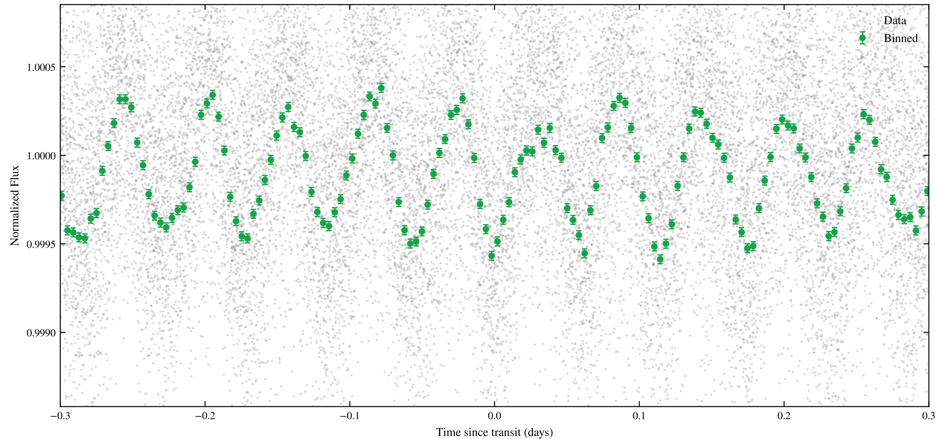
TIC 409934330 | Sectors: 93, 94 | Phase-Folded Transit (P = 0.80289 d)
