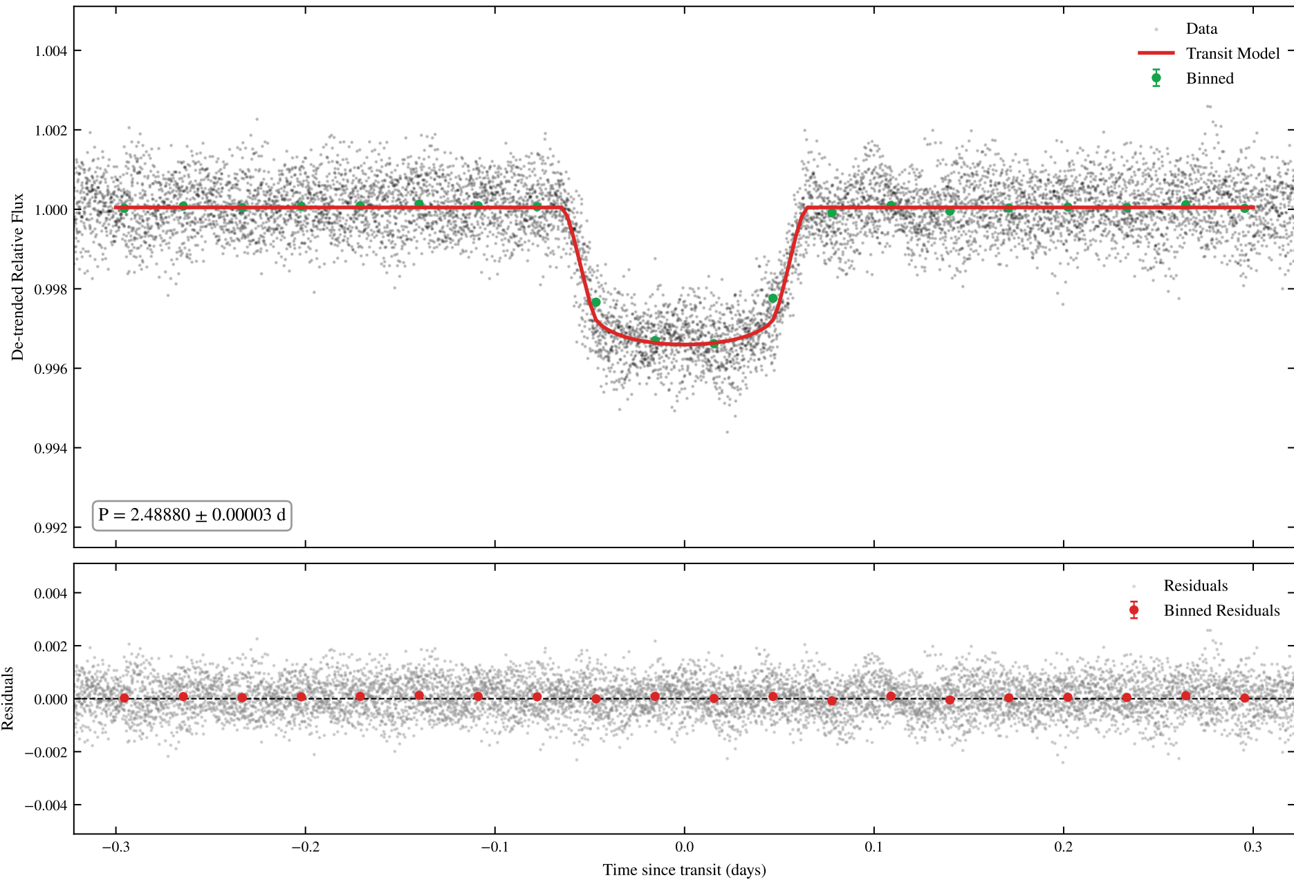
TIC 409934330 | Sectors: 93, 94 | Phased MCMC Fit - Planet 1
