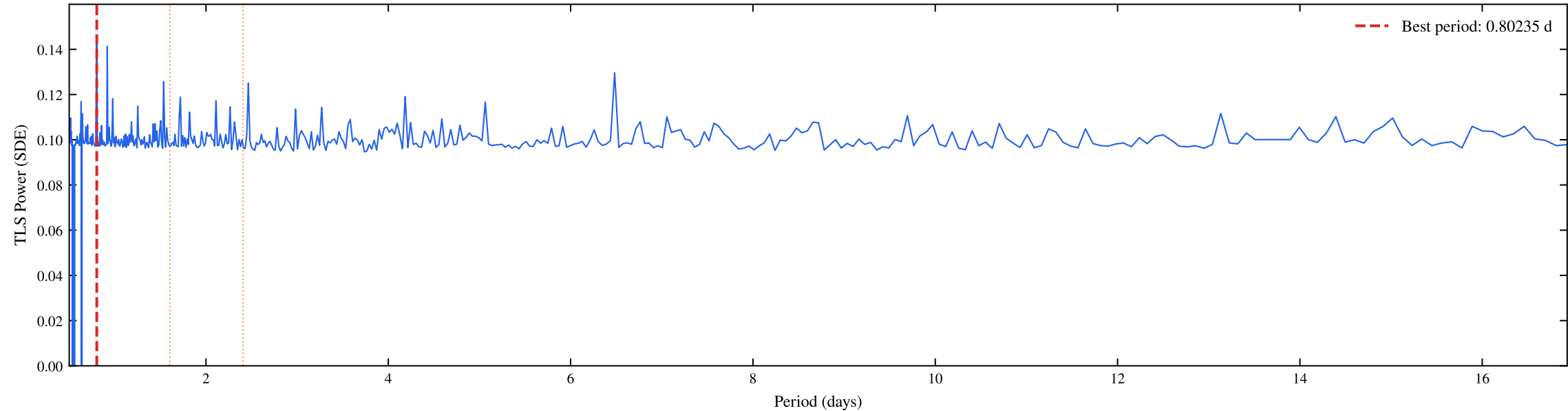
TIC 409934330 | Sectors: 93, 94 | TLS Coarse Periodogram (SDE = 0.15)
