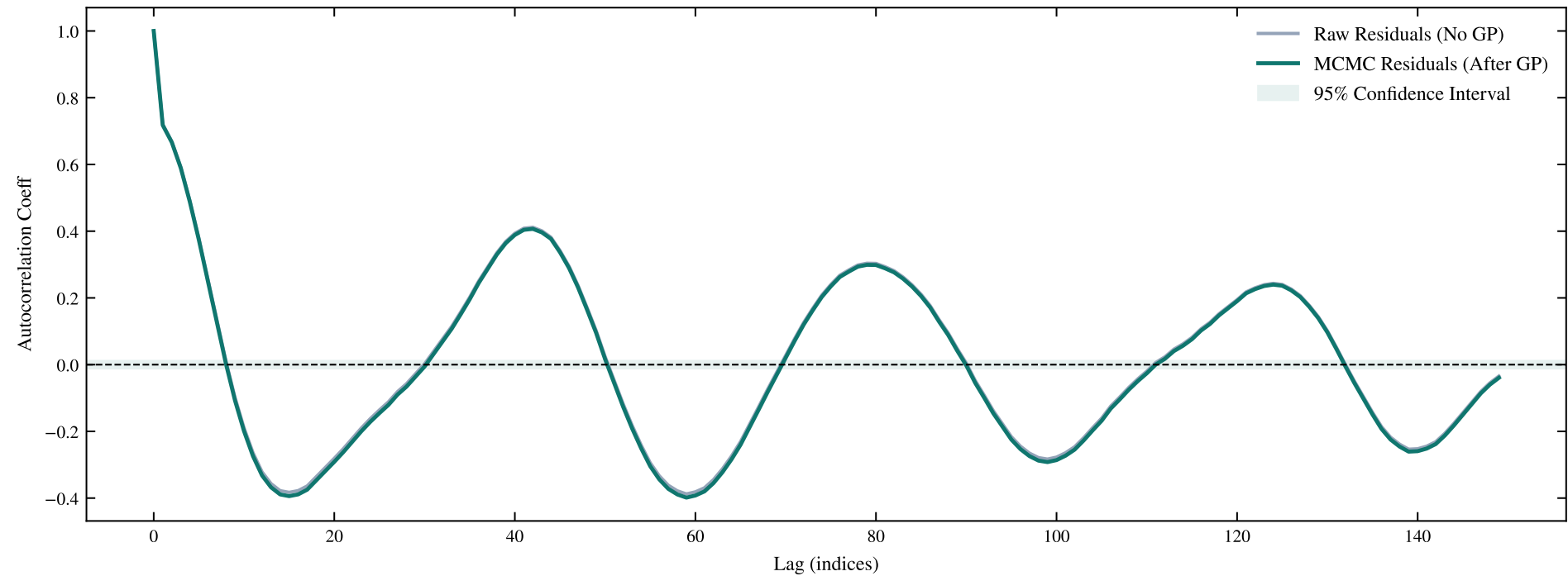
TIC 409934330 | Sectors: 93, 94 | GP Residuals Autocorrelation Function (ACF)
