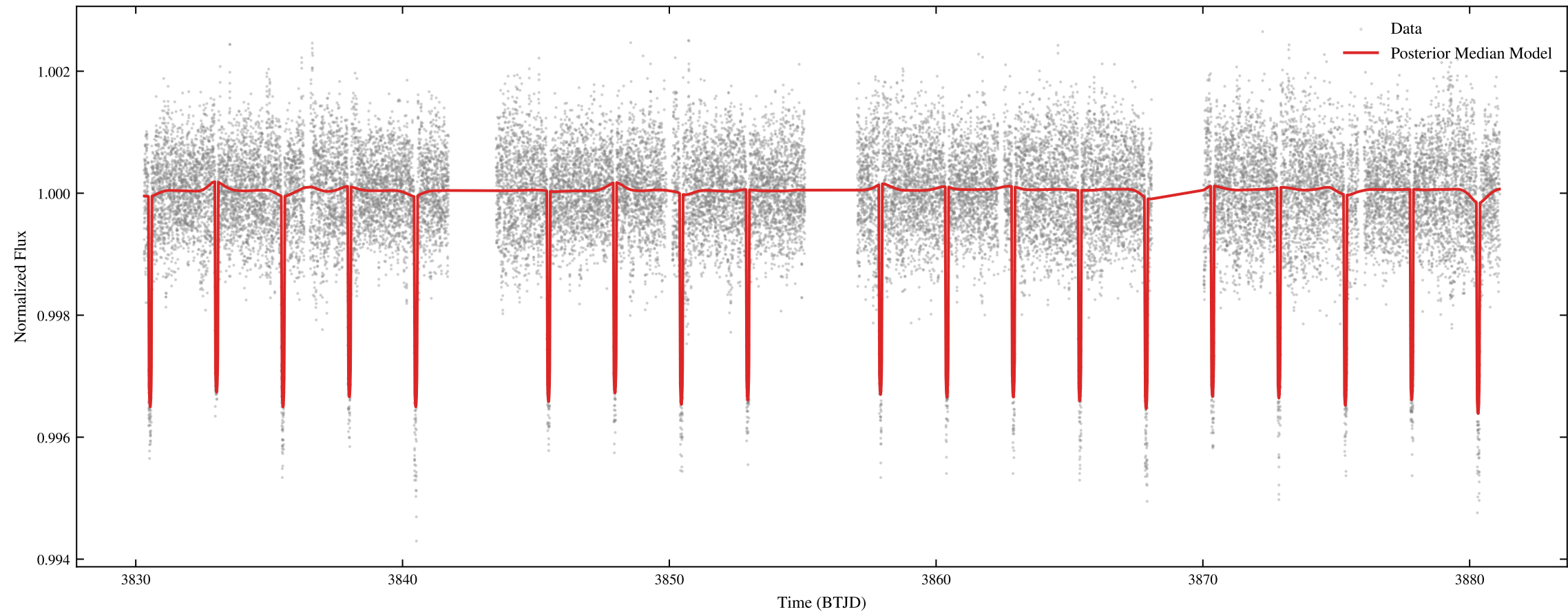
TIC 409934330 | Sectors: 93, 94 | MCMC Posterior Predictive Check
