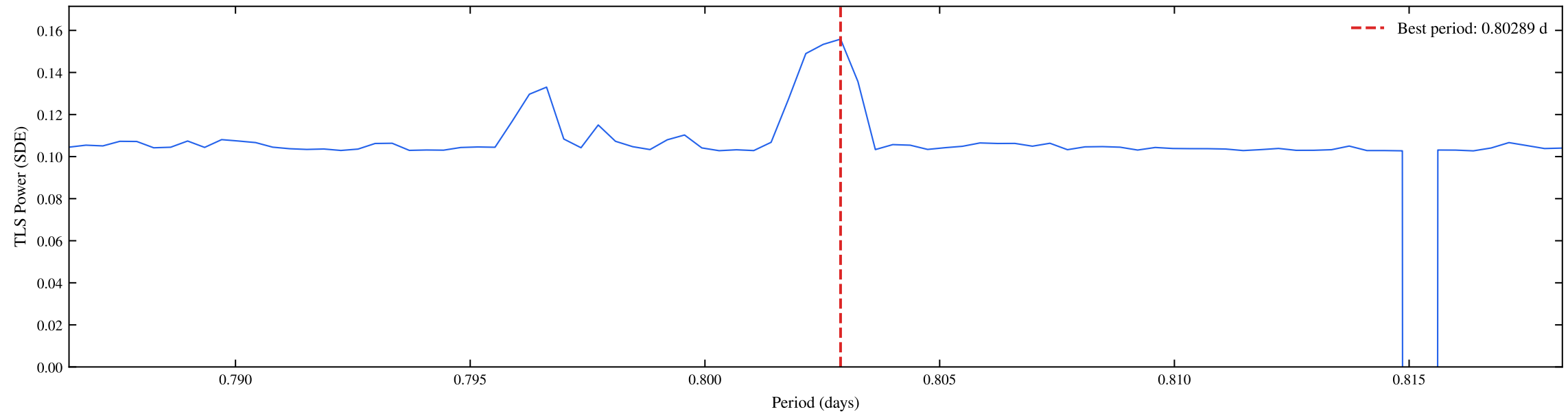
TIC 409934330 | Sectors: 93, 94 | TLS Fine Periodogram (SDE = 0.16)
