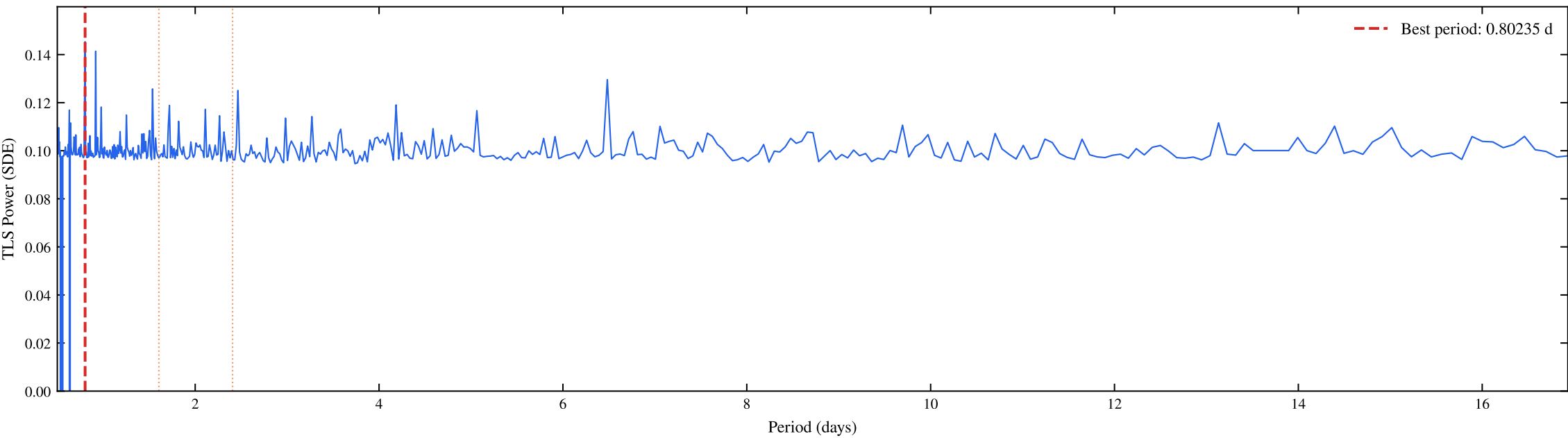
TIC 409934330 | Sectors: 93, 94 | TLS Periodogram (Planet 2 Search) (SDE = 0.15)
