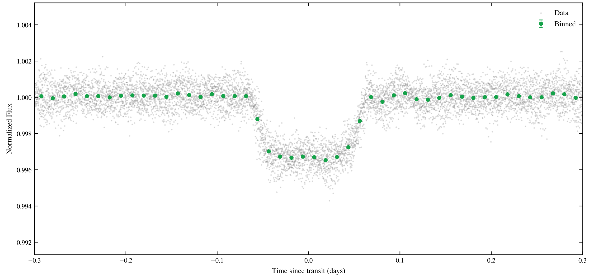
TIC 409934330 | Sectors: 93, 94 | Phase-Folded Transit (P = 2.48885 d)
